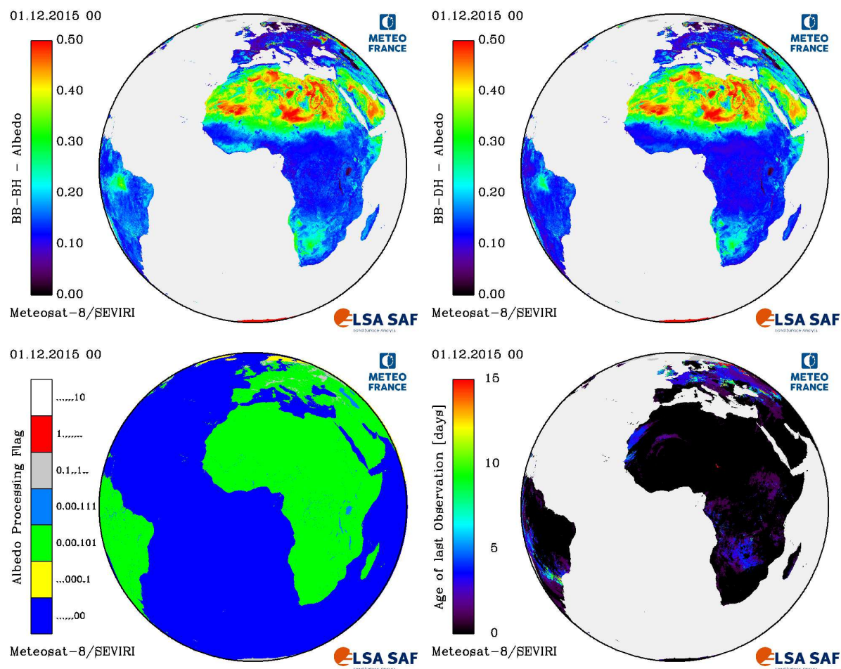
Figure 10: Broad-band albedo product for the 1 st of December 2015.
