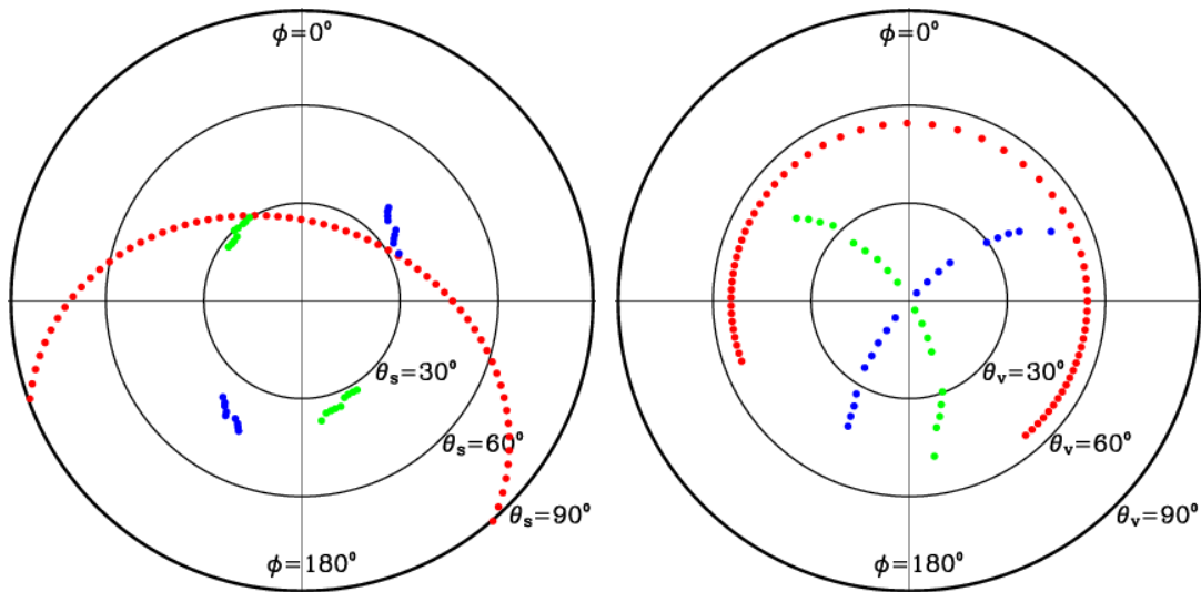
Figure 3: Illumination (left) and observation (right) geometries corresponding to a geographical location of [47° 47' N, 10° 37' E ] and an observation period between the days of year 150 and 170.
