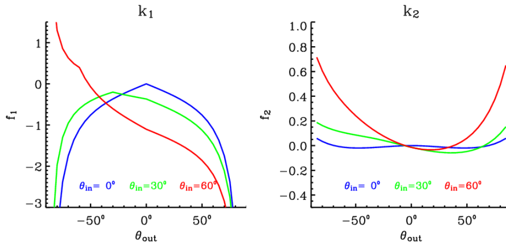
Figure 4: Angular dependence of the “geometric” (left) and “volume scattering” (right) kernels of the reflectance model introduced by Roujean et al. (1992).
