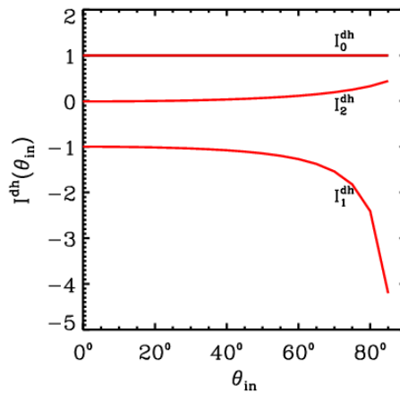
Figure 8: Illumination zenith angle dependence of the directional-hemispherical kernel integrals for the Roujean et al. (1992) model.
