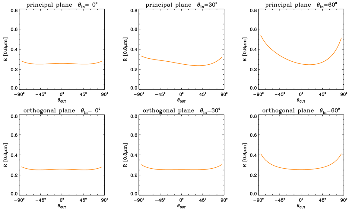
Figure 6: The dependence of the 0.8μm-channel reflectance factor on the direction of the outgoing light ray for different incidence directions according to the model fit of the example case from Figure 5.
