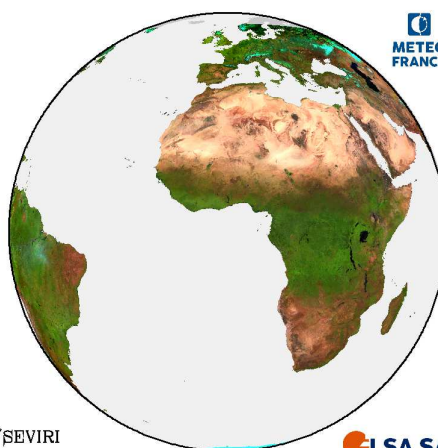
Figure 11: Colour composite derived from the three spectral directional-hemispherical albedo estimates for the 1 st of December 2015.
